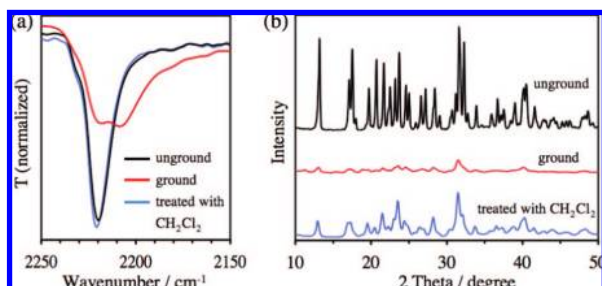
Figure 4. IR and XRD spectra of 1 in various states.
