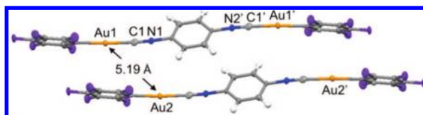
Figure 3. Partial view of the crystal packing of a blue luminescent crystal of 1 . Thermal ellipsoids were drawn at 50%-probability level. Crystal data: monoclinic, P2_1/c (No. 14), a = 5.190(2) Å, b = 17.154(6) Å, c = 10.861(4) Å, \beta = 90.83(3)^\circ , V = 966(2) Å 3 , Z = 2 . T = 296.2 K. 2\theta_{\max} = 55.0^\circ , R = 0.0355 ( I > 2.00\sigma(I) ), R_w = 0.0976 , GOF = 1.007 .
