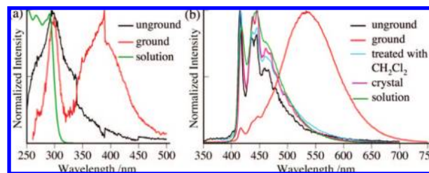
Figure 2. (a) Absorption and (b) emission (excited at 260 nm) spectra of 1 in various states.
