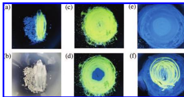
Figure 1. Photographs showing Au(I) complex 1 on an agate mortar under UV irradiation with black light (365 nm), unless otherwise noted: (a) Au(I) complex 1 powder after grinding the right-half with a pestle, (b) same sample under ambient light, (c) entirely ground powder of 1 , (d) partial reversion to the blue luminescence by dropwise treatment using dichloromethane onto the center of the ground powder, (e) powder after treatment with dichloromethane, and (f) repetition of the yellow emission by scratching the powder with a pestle (see video 1 for a movie of the grinding process).
